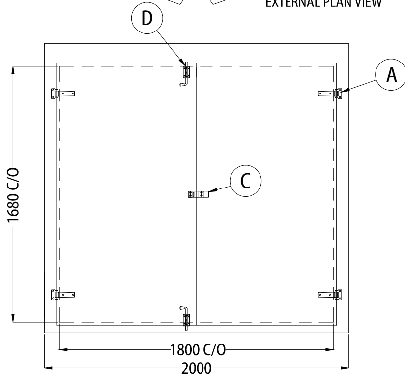
EXTERNAL VIEW ON FRONT WALL
