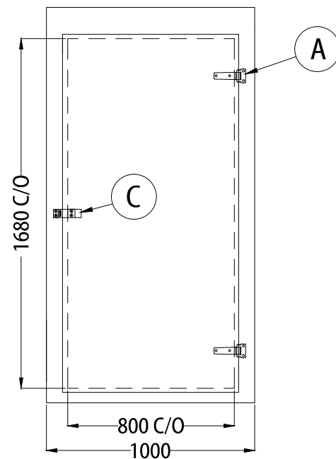
EXTERNAL VIEW ON FRONT WALL
